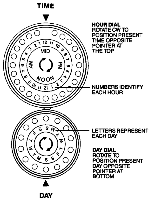
Figure 5 CONTROLLER CLOCK
